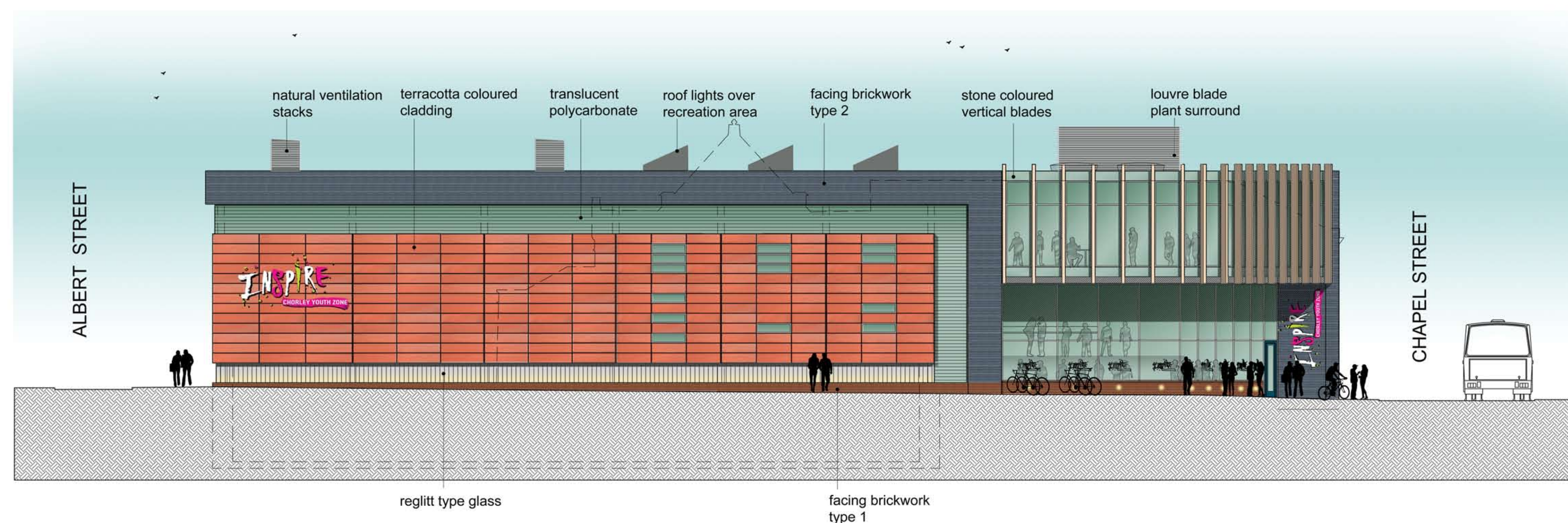
RAILWAY STREET ELEVATION
